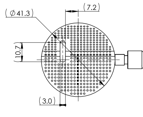
60µ/70µ PERFORATED COVER PHA UMB LENGTH = 3m (OPTIONAL)
